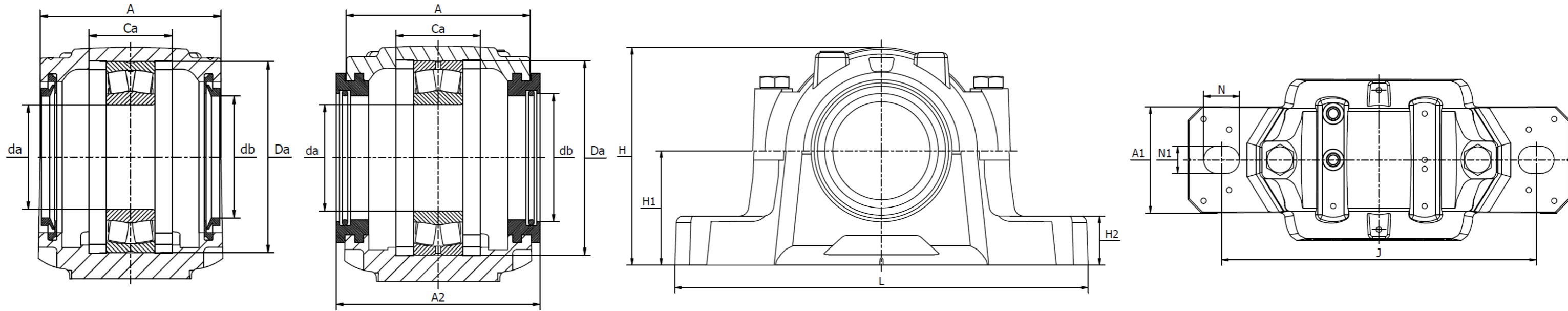
Felt seal, Rubber seal and V-ring seal
