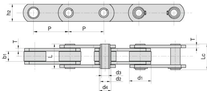
without rollers
