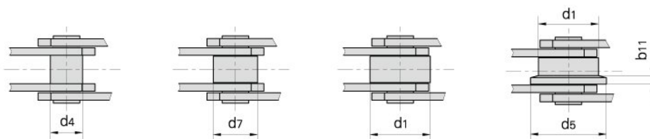
without rollers
