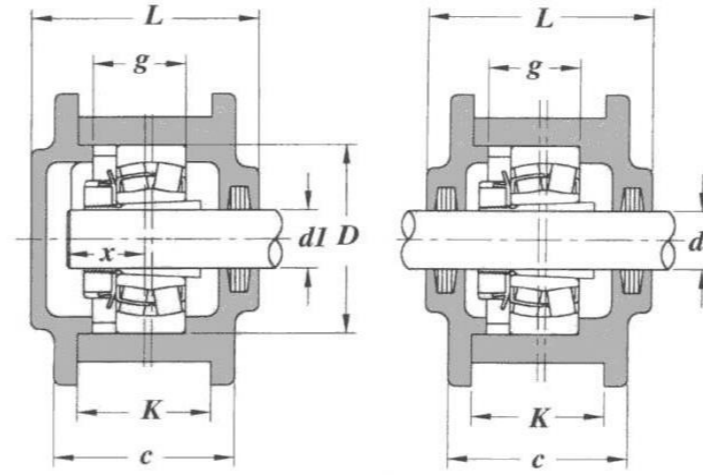
Housing for shaft end. A Type
