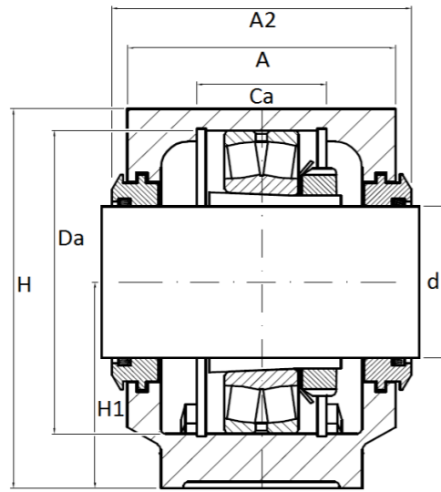
Labyrinth seal
